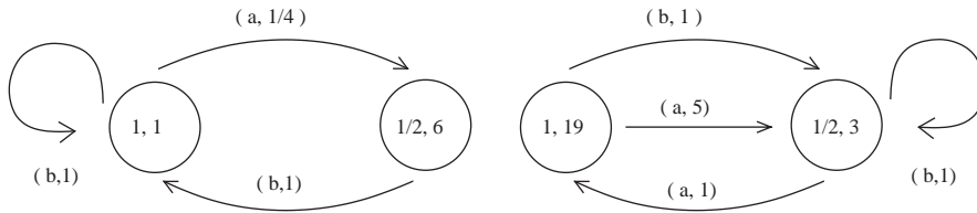
Fig. 3. Two weighted finite automata over the alphabet \{a, b\} , defining the primitive linear representations (\pi_i, v_i, \tau_i) , i = 1, 2 .
