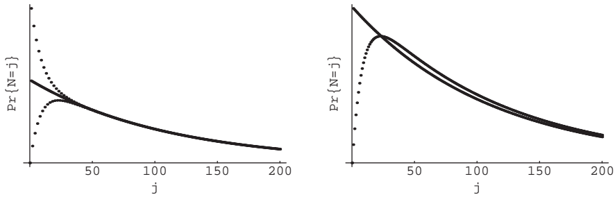
Fig. 1. Probability law of the random variable N defined in (36), for j = 0, 1, \dots, 200 . In the first picture we compare the case \mu = 0.00001 and -0.89 . In the second one we compare the case \mu = 0.00001 and +0.89 .
