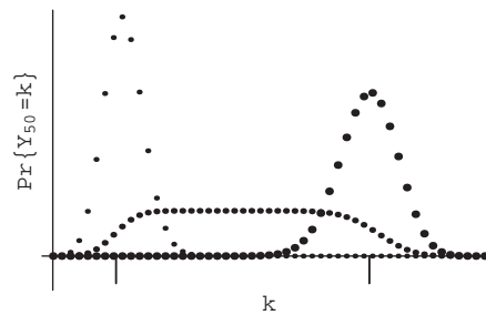
Fig. 4. Probability functions of Y_{50} in the product model where the two factor components are defined by Fig. 3 with weighted expanded by a constant factor. The vertical bars have abscissas 50\beta_1 and 50\beta_2 . The curves correspond to the cases where (\lambda_1, \lambda_2) are equal to (2,1), (1,2) and (1,1), respectively.
